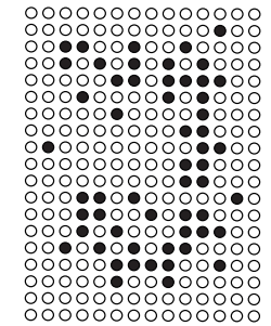
INPUT PATTERN
