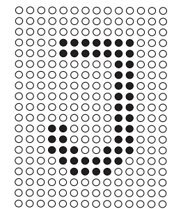
SAVED PATTERN
