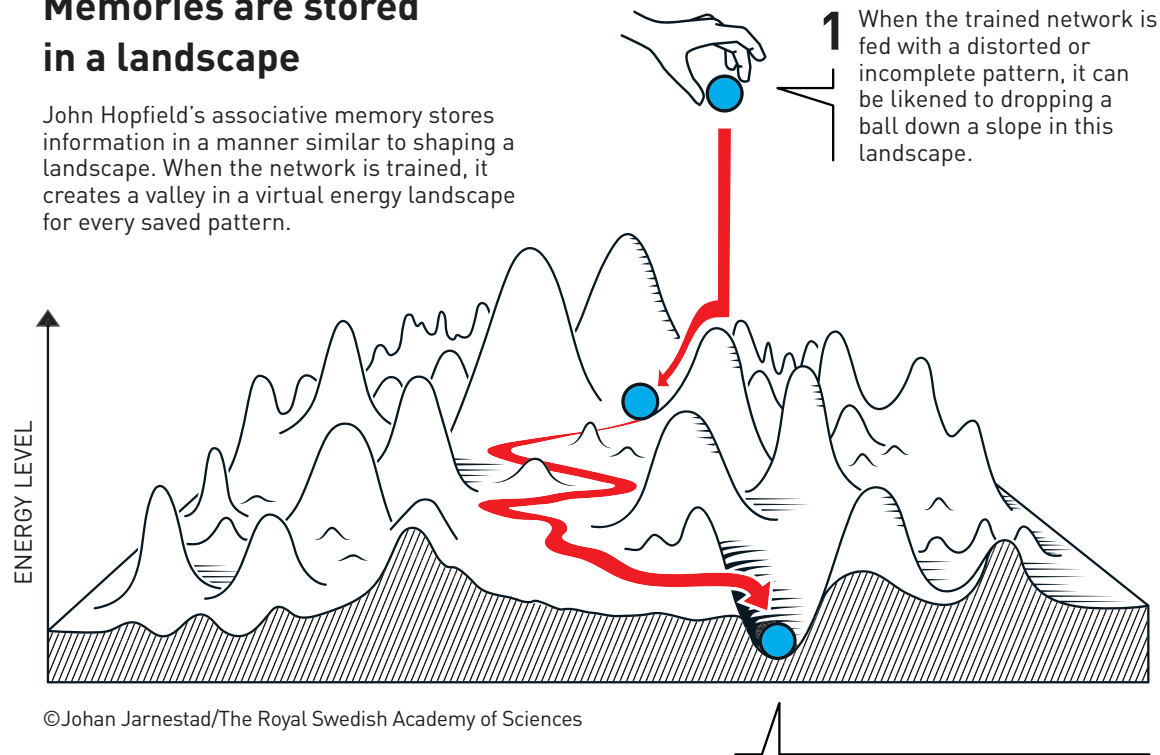
SAVED PATTERN
